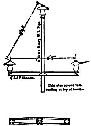
FIG. 5.—SPECIAL FOUR-POST LINE TOWER, GUANAJUATO POWER & ELECTRIC COMPANY.
